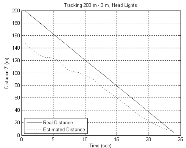
Fig. 12. Distance estimation 200 - 0 m. Head lights
