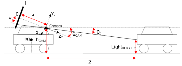
Fig. 6. Vertical road and mapping geometry
