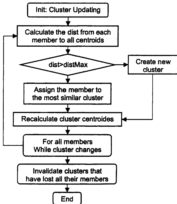
Fig. 4. Description of the 'k-means' clustering algorithm.
