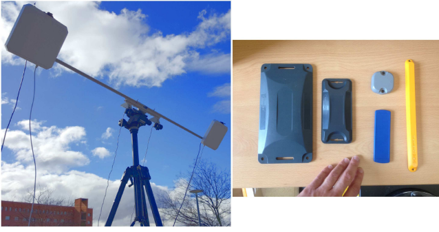
Fig. 4. Left: sensor setup, including two CMOS USB cameras and two far field circularly polarized panel antennas within the 865-870MHz band (Europe frequency allocation) located at the same baseline. Right: different passive RFID tags used in our experiments.
